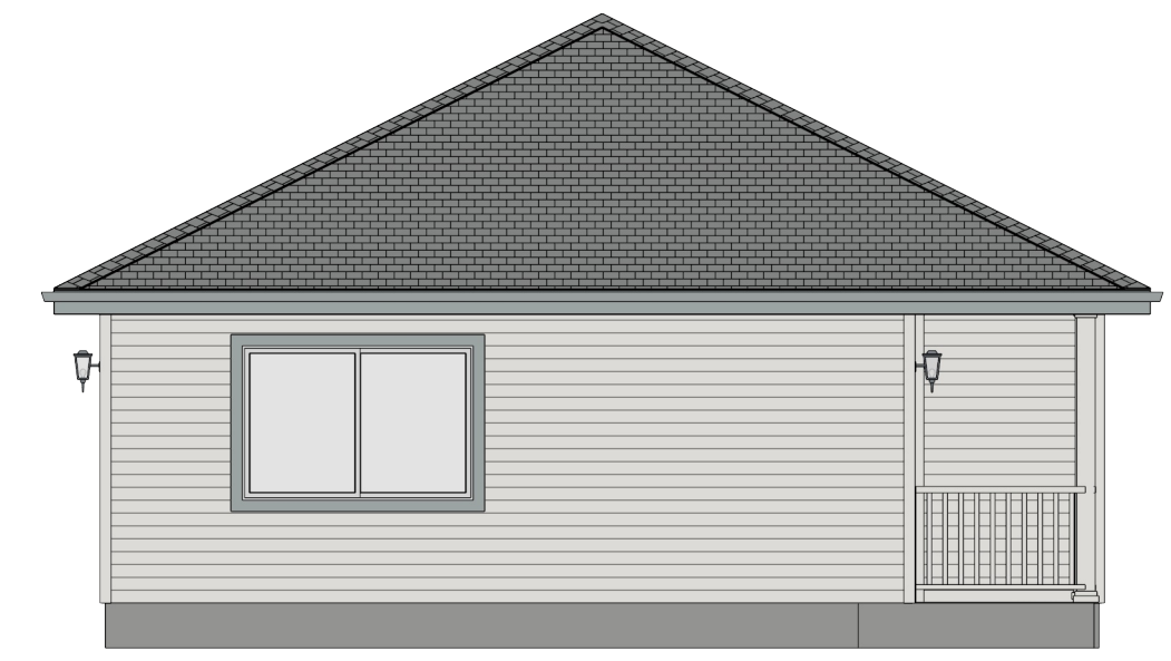
Left Elevation
